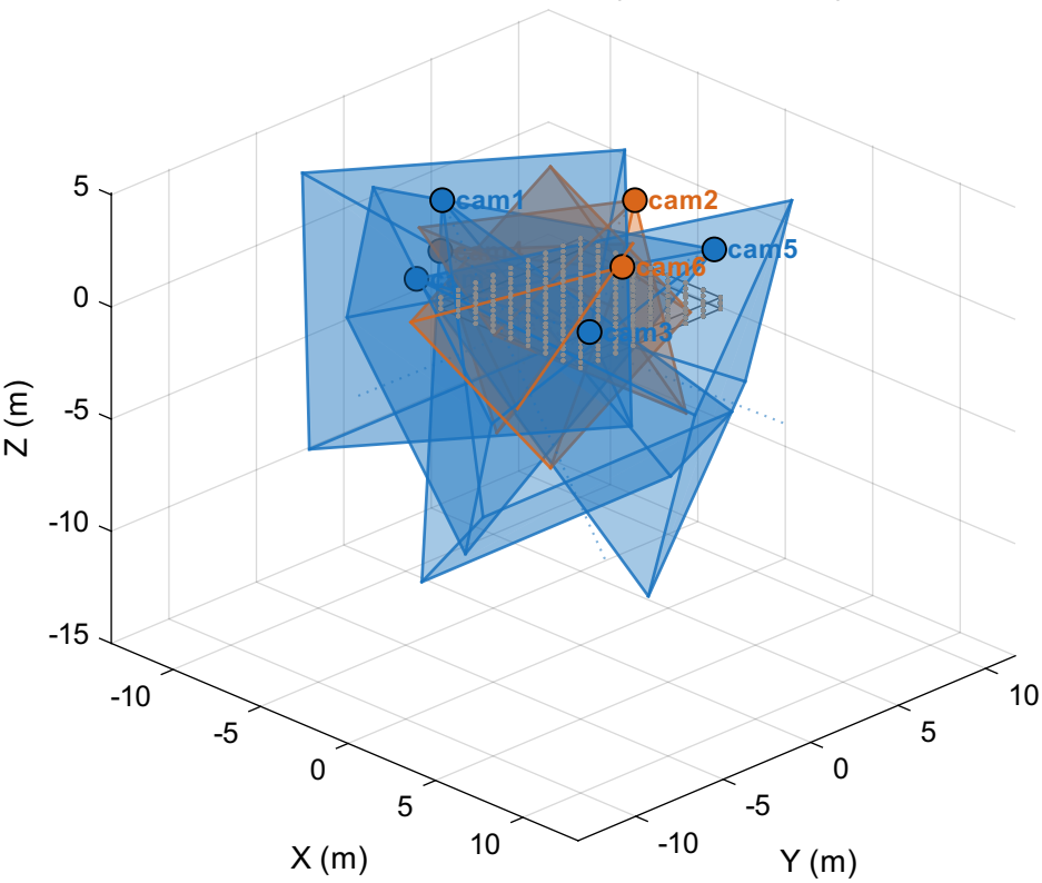
GA-best — 7 cams (Cost: 0.0179)
